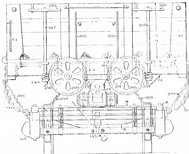
Fig. 338. End Elevation.
